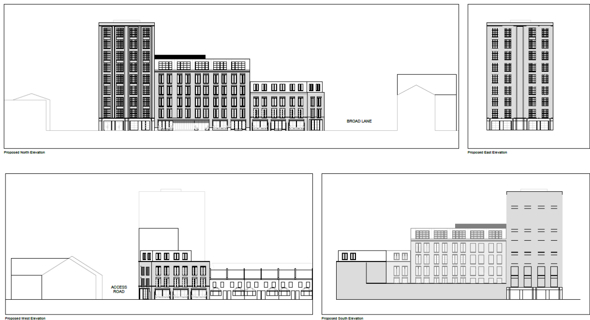
Proposed elevations
